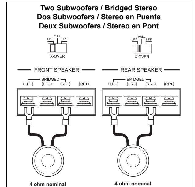
2-Channel Mode
